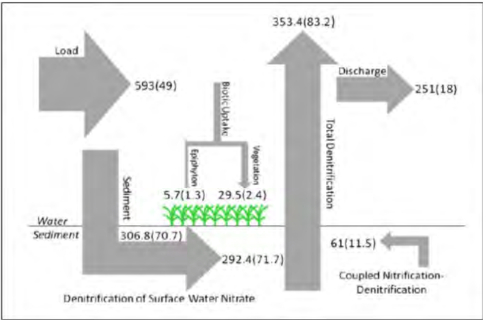
Figure 26. Net \text{NO}_3\text{-N} budget (mean (1 SE), \text{mg m}^{-2} \text{h}^{-1} ) for Third Lake, Navigation Pool 5 during June and July 2005. n = 3 for discharge and load, n = 8 for coupled nitrification–denitrification and total denitrification, n = 16 for biotic uptake and denitrification of surface water nitrate. Reprinted from Kreiling et al. (2010).
