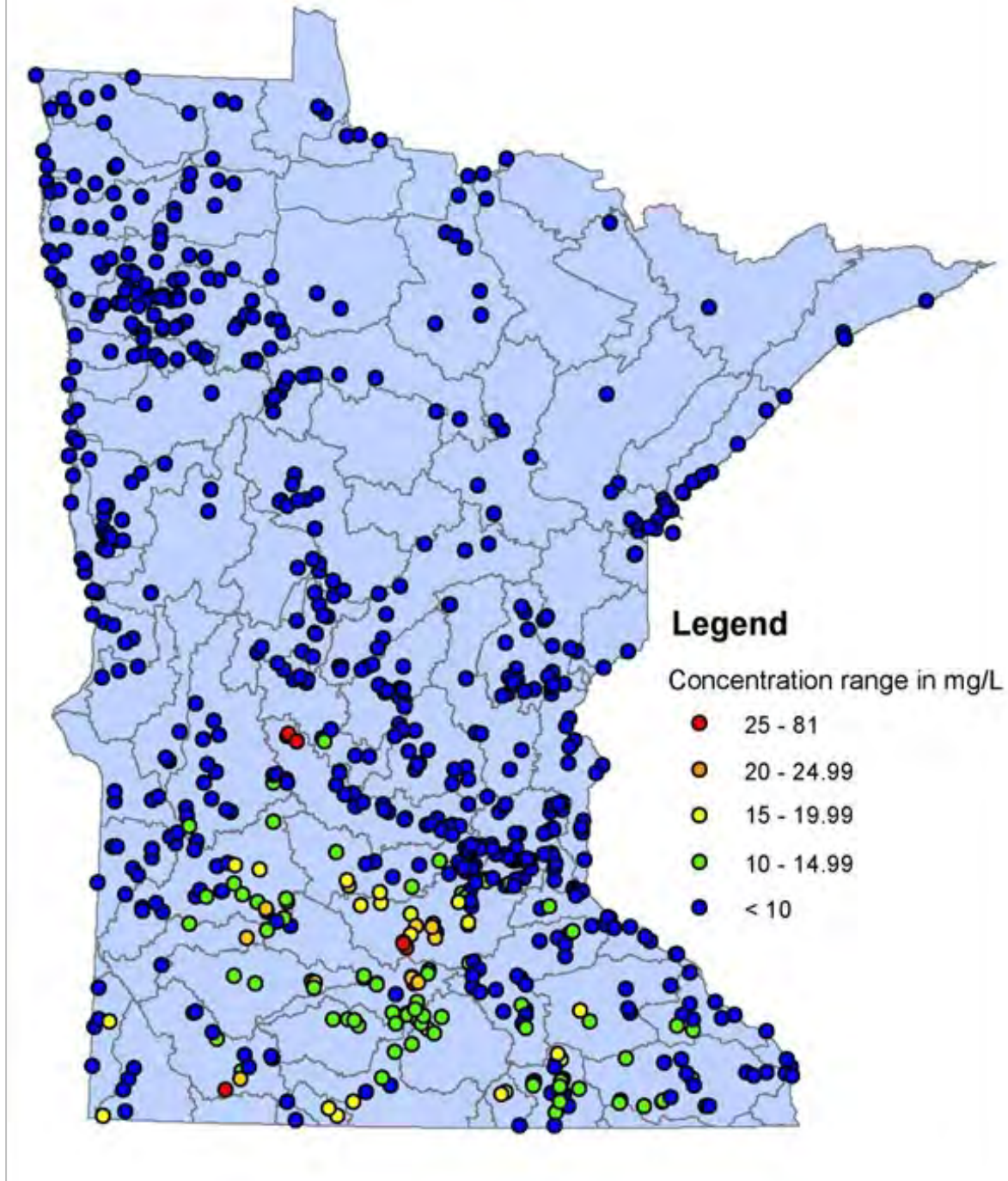
Figure 2. Nitrite+Nitrate-N 90 th percentile concentrations, showing the magnitude of 90 th percentile concentrations greater than 10 mg/l. This is the same figure as Figure 1, except that the concentration scale ranges are different, such that all red shaded points in Figure 1 are subdivided into four separate categories.
