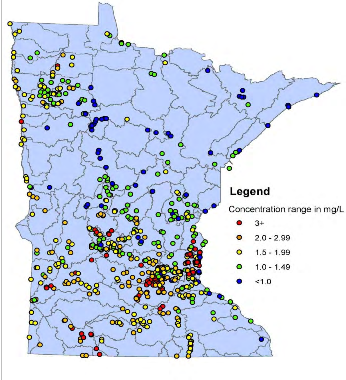
Figure 8. 90 th percentile TKN concentrations for all samples taken at each site between 2000 and 2010.
