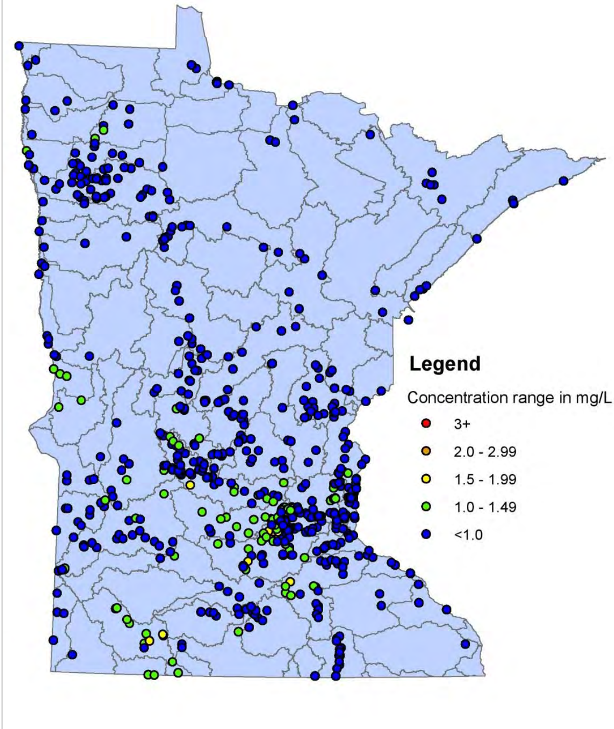
Figure 10. 10 th percentile TKN concentrations for all samples taken at each site between 2000 and 2010.
