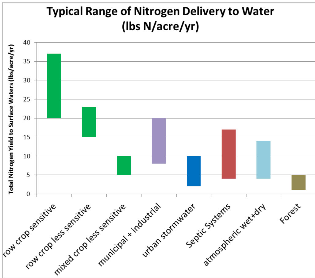
Figure 19. Graphical depiction of the source yield ranges from Table 6. Average precipitation year.
