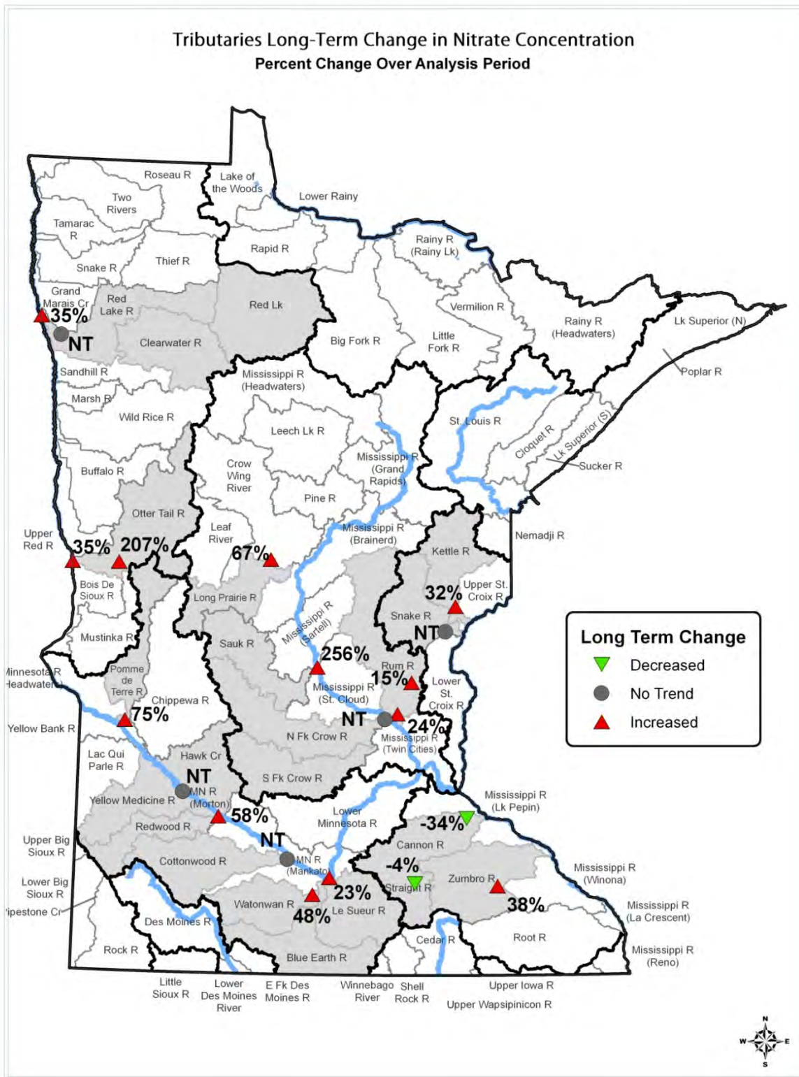
Figure 4. Percent change of nitrate concentrations in tributary rivers during the entire period of analysis (typically 1976 to 2010, but varied by site - see Tables 2 to 16). Watersheds associated with the trend analyses are shaded in gray.
