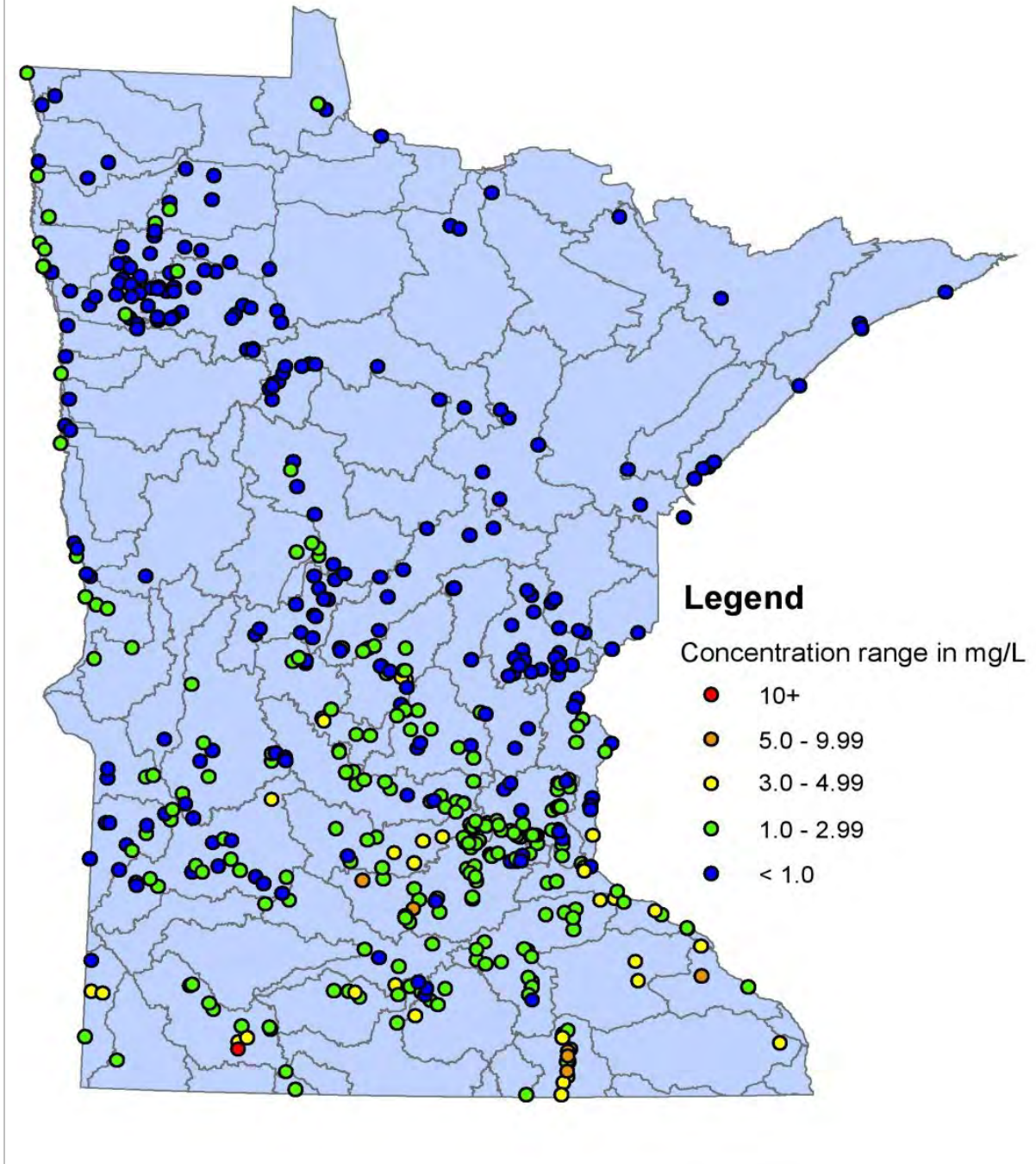
Figure 13. 10 th percentile TN concentrations for all samples taken at each site between 2000 and 2010.
