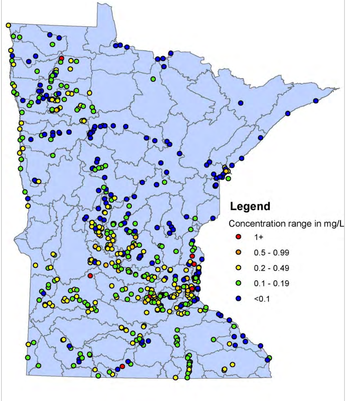
Figure 5. 90 th percentile ammonia+ammonium-N concentrations for all samples taken at each site between 2000 and 2010.
