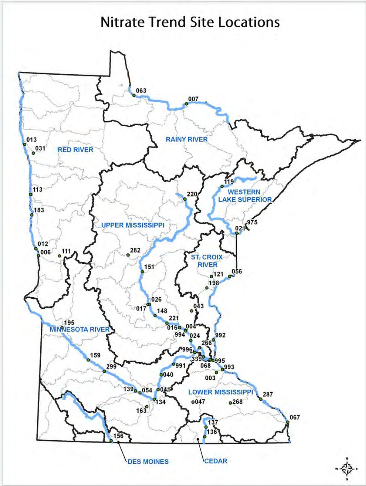
Figure 1. Site locations and associated site numbers for each of the river monitoring sites where trend analyses were completed (refer to Table 1 for more information about each site).
