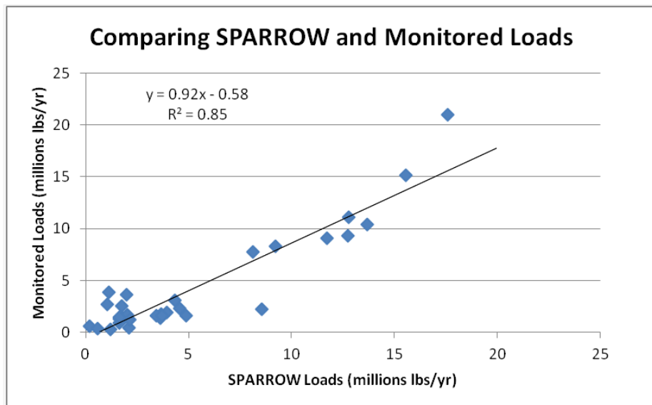
Figure 9. HUC8 watershed outlet SPARROW modeled loads plotted against monitoring-based load estimates developed from the average of two typical flow years between 2005 and 2009.
