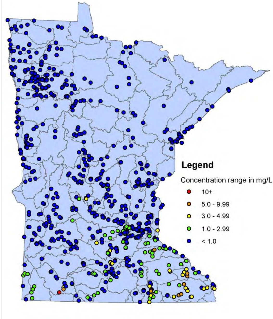
Figure 4. Nitrite+nitrate-N 10 th percentile concentrations for all samples taken at each site between 2000 and 2010.
