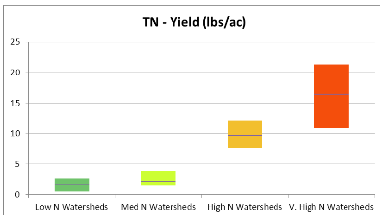
Figure 7. Total nitrogen annual yield from the 28 study watersheds. Monitoring and yield calculations conducted by the MPCA and Metropolitan Council.
